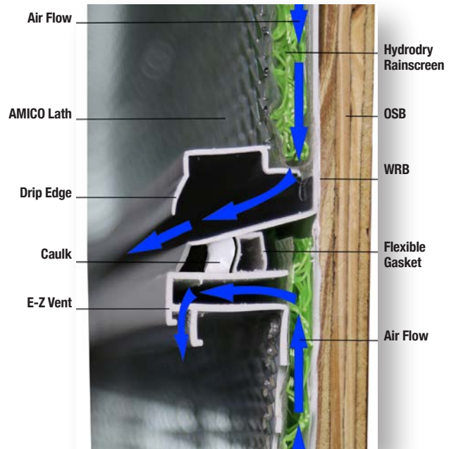
Create a Fully Vented/Drainable Midwall by Combining EZ-Vent and the Amiflow Drip Edge
