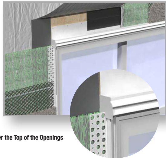
Create a Fully Vented/Drainable Midwall by Combining EZ-Vent and the Amiflow Drip Edge
