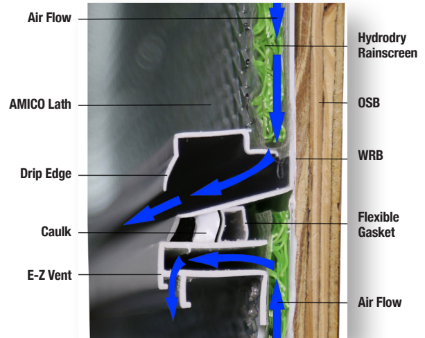
Create a fully vented/drainable midwall by combining EZ-Vent and the Amiflow Drip Edge
