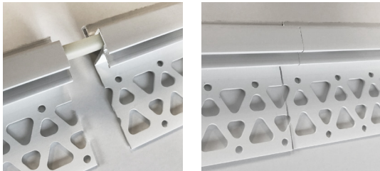
The E-Z Vent connector allows installers to attach pieces of E-Z Vent profiles to create a continuous seamless profile that lines up perfectly every time.
