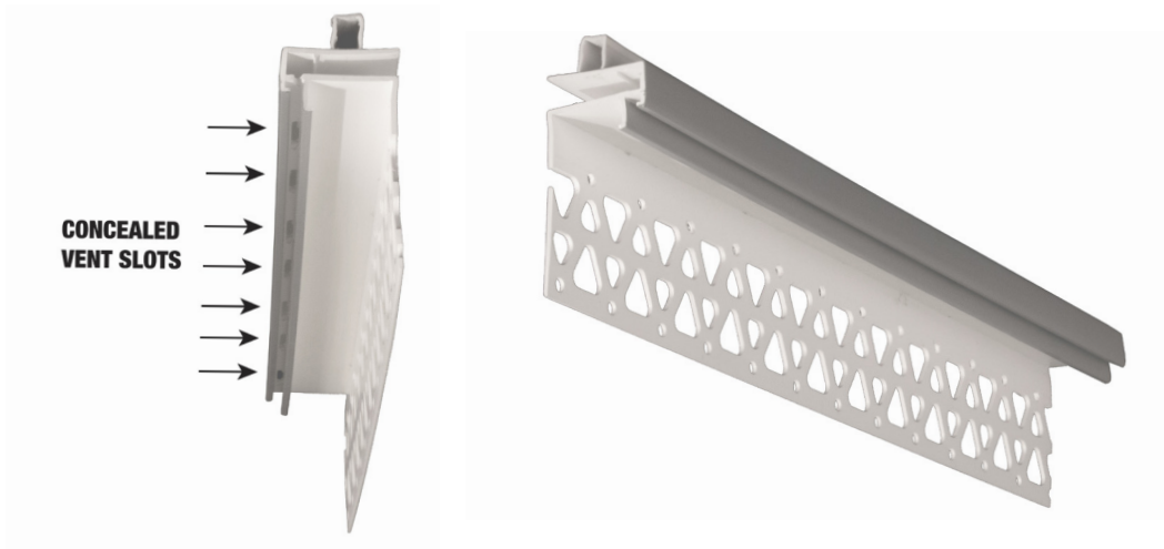
E-Z Vent's concealed vent slots allow air and water vapor to escape from within the interior cavity out the top of the wall
